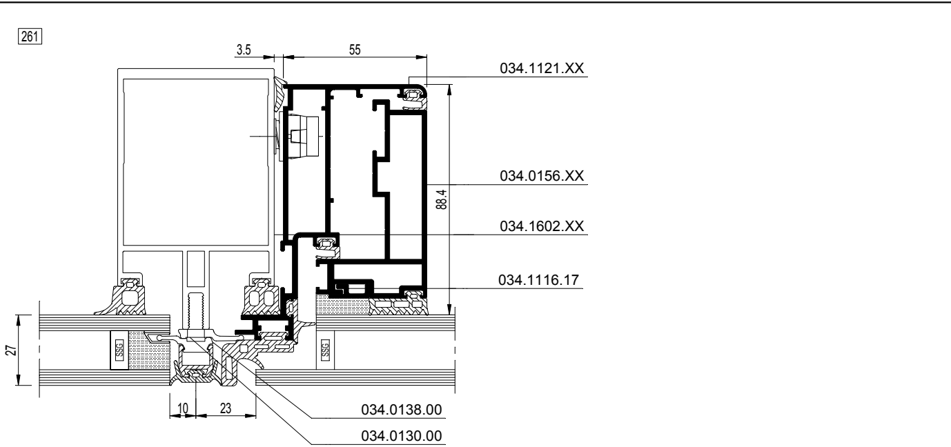
CW60-261003.dxf CW60-261003.dwg
